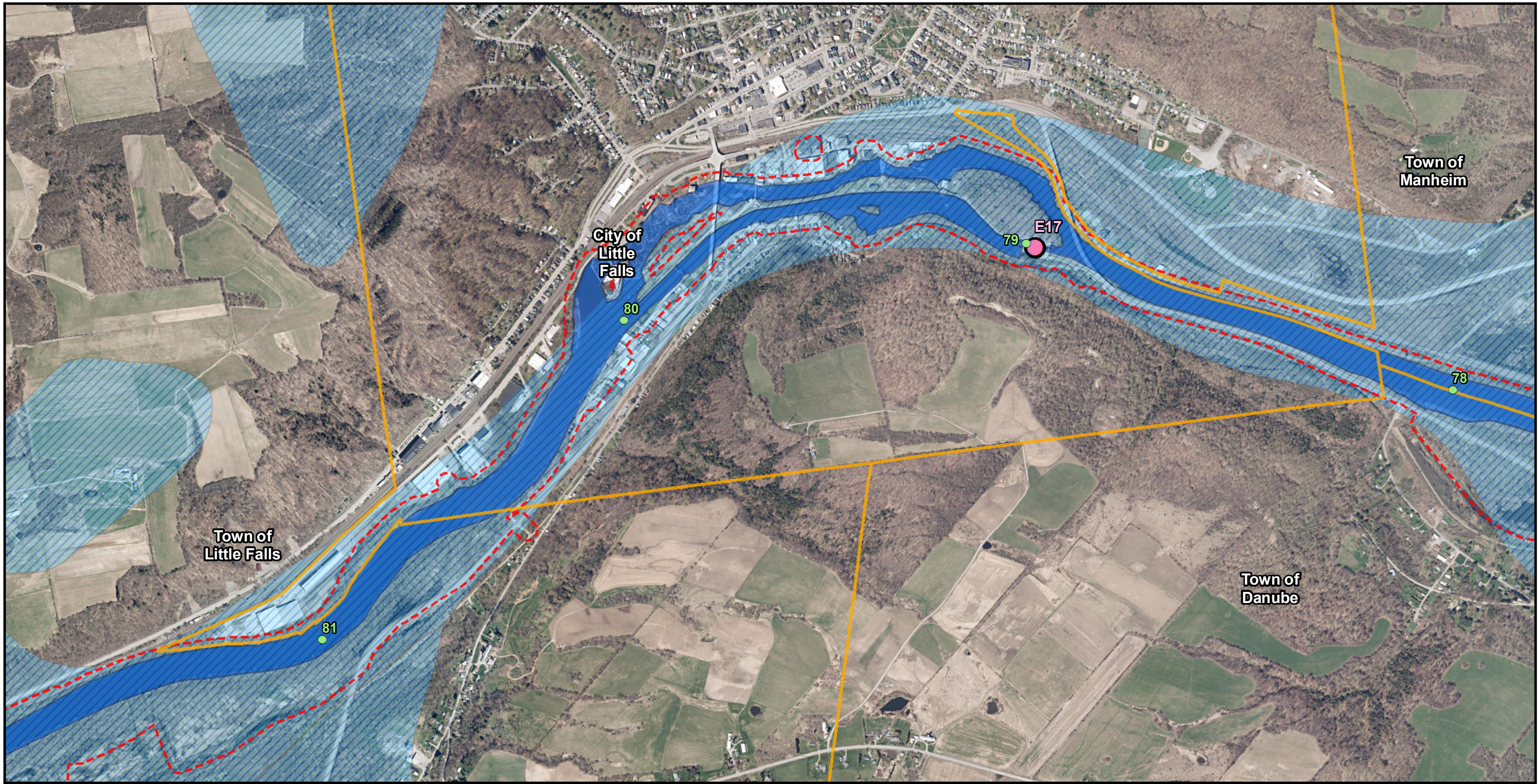
Figure 39F: Aquifers
